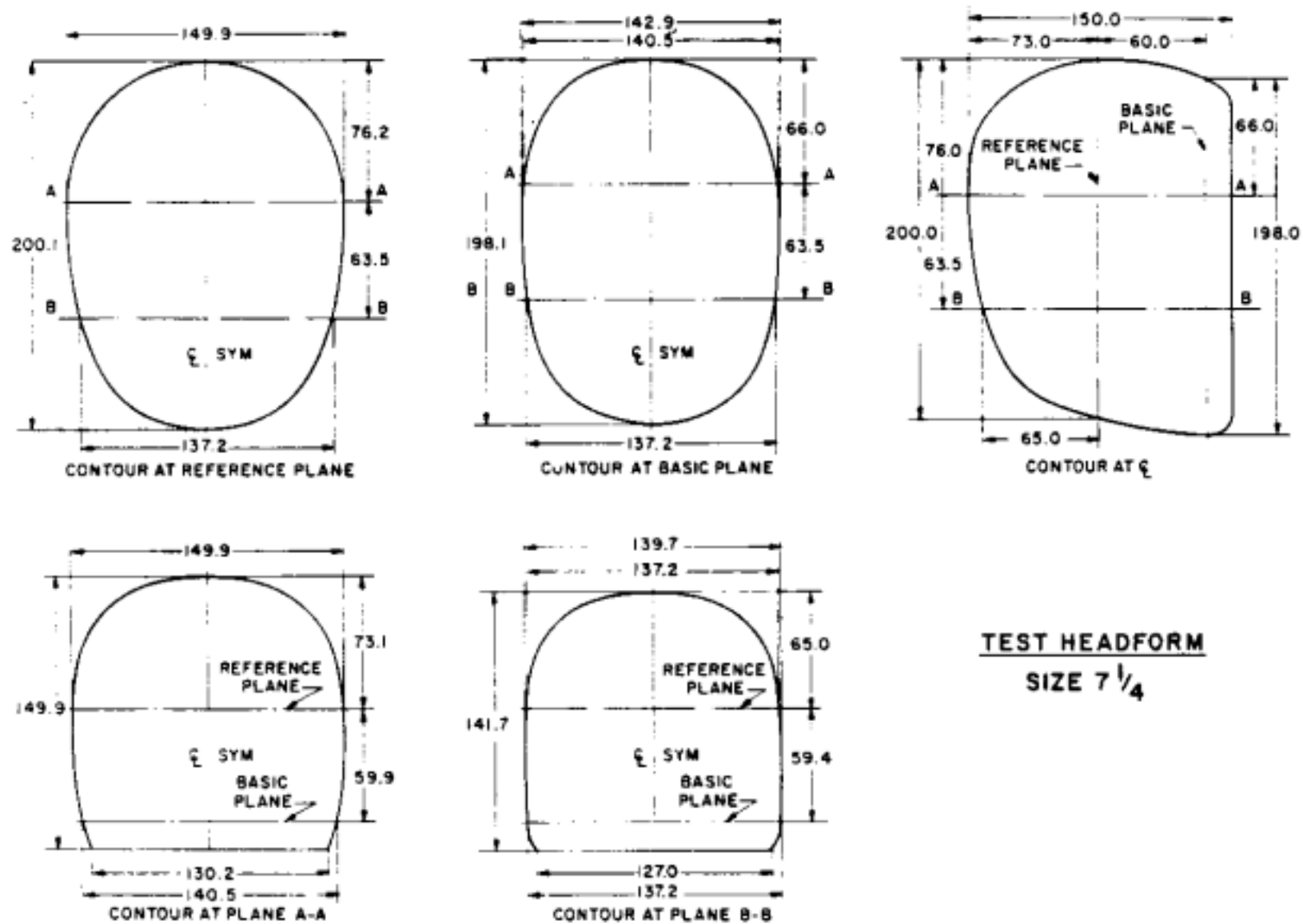
Figure 3. Test headform. Dimensions are in millimeters.
