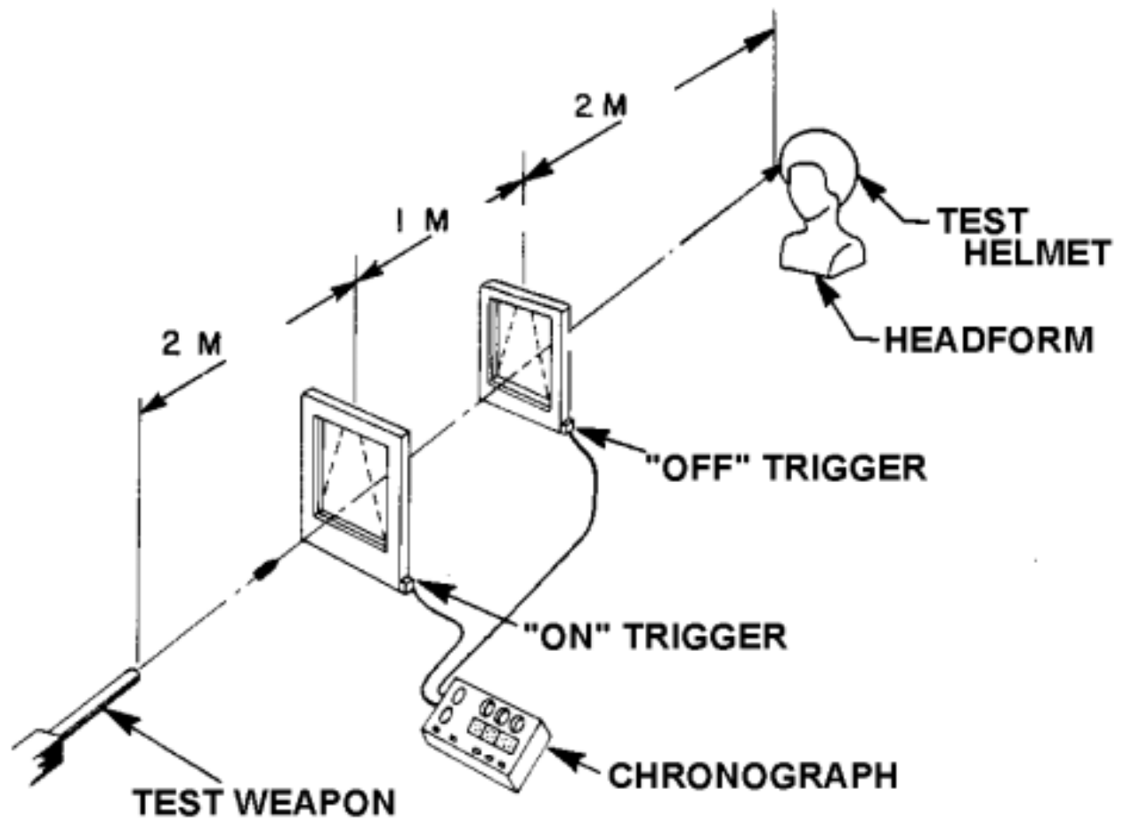
Figure 6. Test setup.
